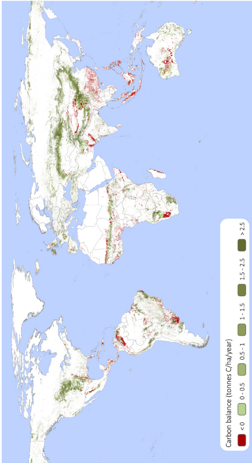
MAP 5 Carbon balance (tonnes C/ha/year) for improved grassland systems
