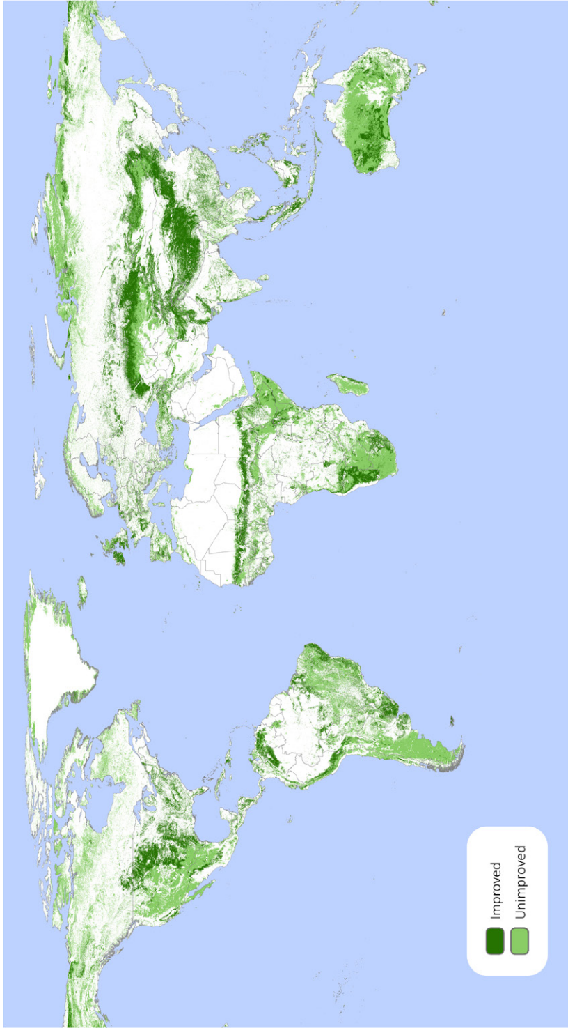
MAP 1 Spatial distribution of unimproved and improved grassland systems
